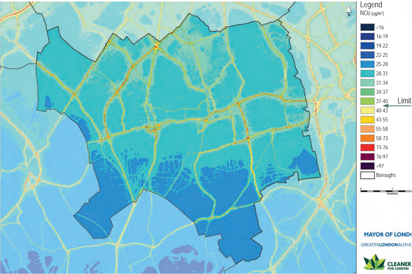
Figure 7 Annual Mean NO 2 Concentrations 2013
